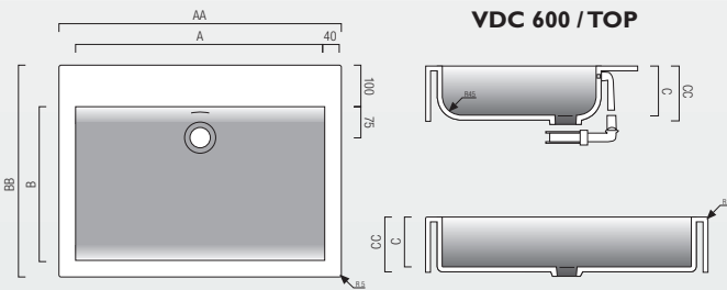
VDC 600 / TOP
